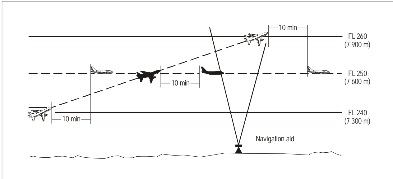
Figure 5-19A. Ten-minute separation between aircraft climbing and on crossing tracks (see 5.4.2.2.2 b))
