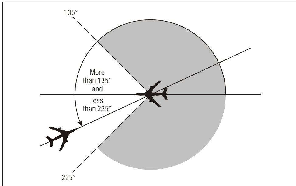
Figure 5-7. Aircraft on reciprocal tracks (see 5.4.2.1.5 b))
