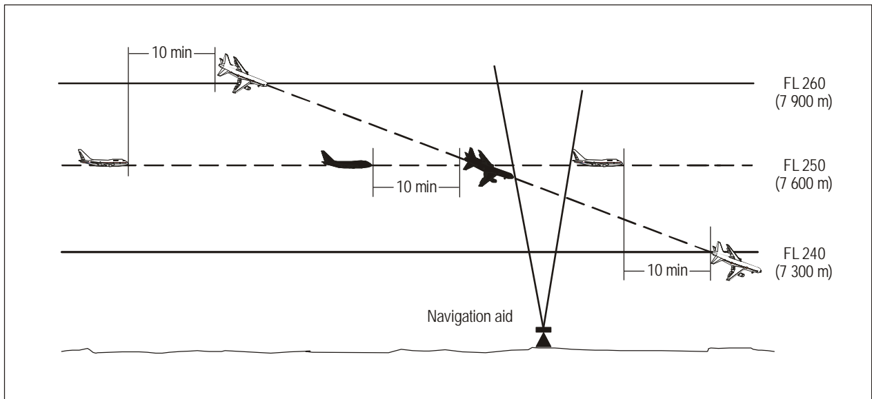
Figure 5-19B. Ten-minute separation between aircraft descending and on crossing tracks (see 5.4.2.2.2 b))
